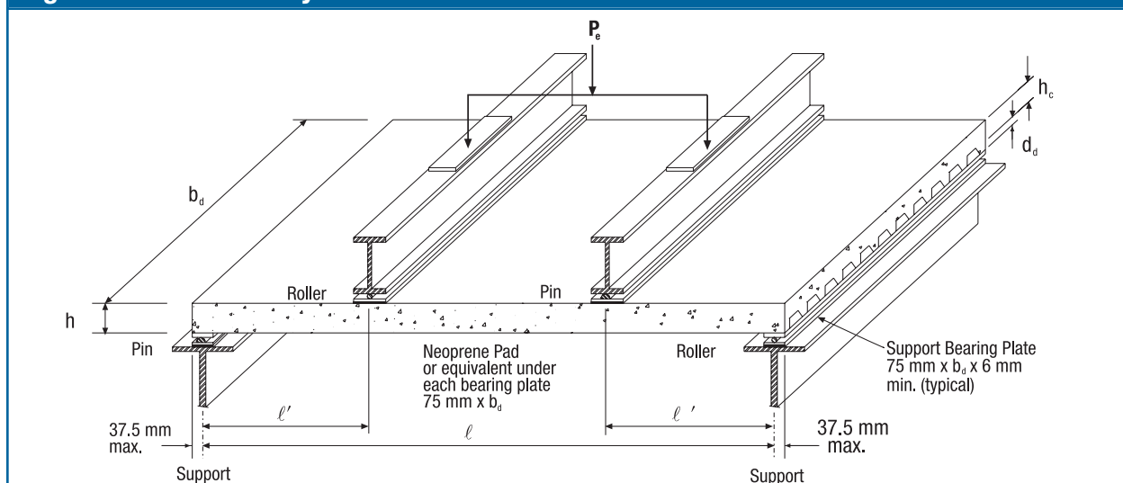
Figure 1: Test Assembly
