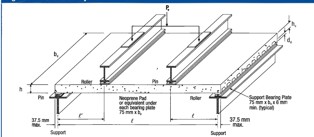
Figure 1: Test Assembly
